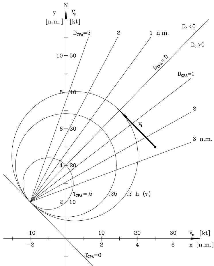
Fig. 2. Lines D_{CPA}=\text{const.} and circles T_{CPA}=\text{const.} \tau=0.2 \text{ h} , X=Y=5 \text{ n.m.} , V_{tx} = -10 \text{ kt} , V_{ty} = 10 \text{ kt}
