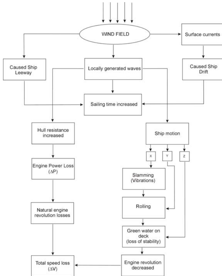
Fig. 2. Environmental effects on speed loss during sea passage in rough seas [6]
