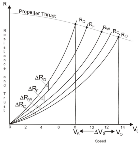
Fig. 4. The ship speed changes due to environmental conditions
