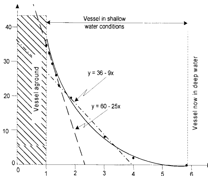
Fig. 6. Loss in speed in shallow water [1]
