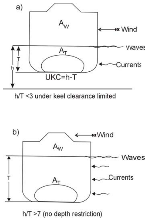
Fig. 3. Different ship's curves reaction on environmental conditions: a) navigation in restricted water areas (ferry); b) navigation in open water areas (bulk carriers) [7]
