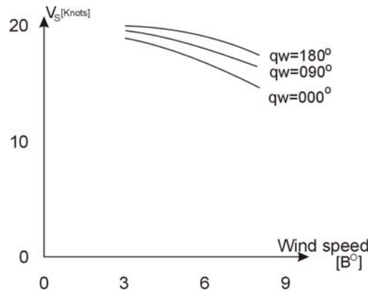
Fig. 7. The ship speed in knot against the wind speed in Beaufort scale
